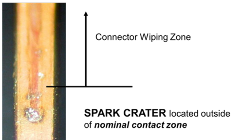
Figure 5. Typical effect of electrical discharge
