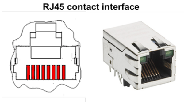
Figure 6. RJ45 contact design
