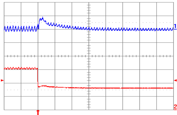
Fig. 0.7525V.8: Output voltage response for V_{out} = 0.7525\text{ V} to negative load current step change from 5 A to 2.5 A with slew rate of -5\text{ A}/\mu\text{s} at V_{in} = 5\text{ V} . Top trace: output voltage (100 mV/div.); Bottom trace: load current (2 A/div.). C_o = 47\text{ }\mu\text{F} ceramic + 1\text{ }\mu\text{F} ceramic. Time scale: 20 \mu\text{s} /div.
